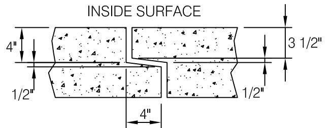
TYPICAL JOINT DETAIL
