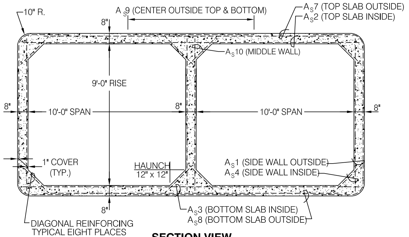
SECTION VIEW
