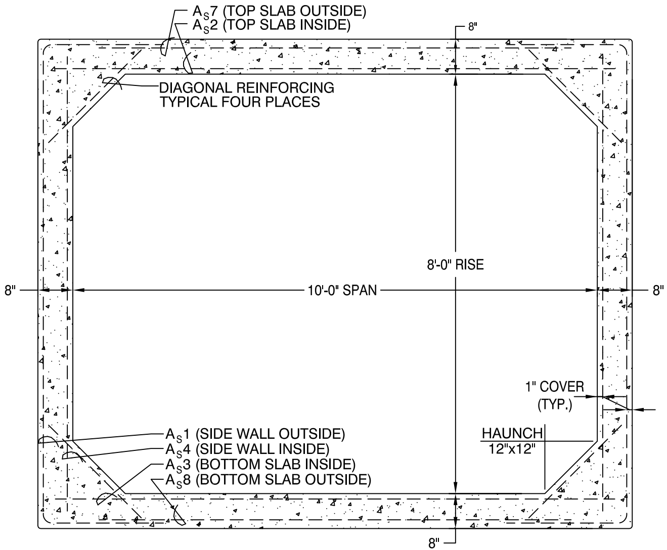
SECTION VIEW
