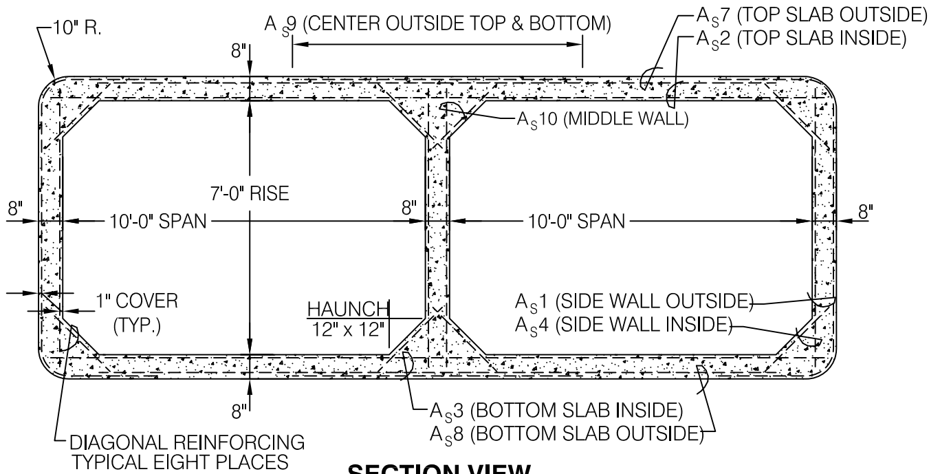
SECTION VIEW
