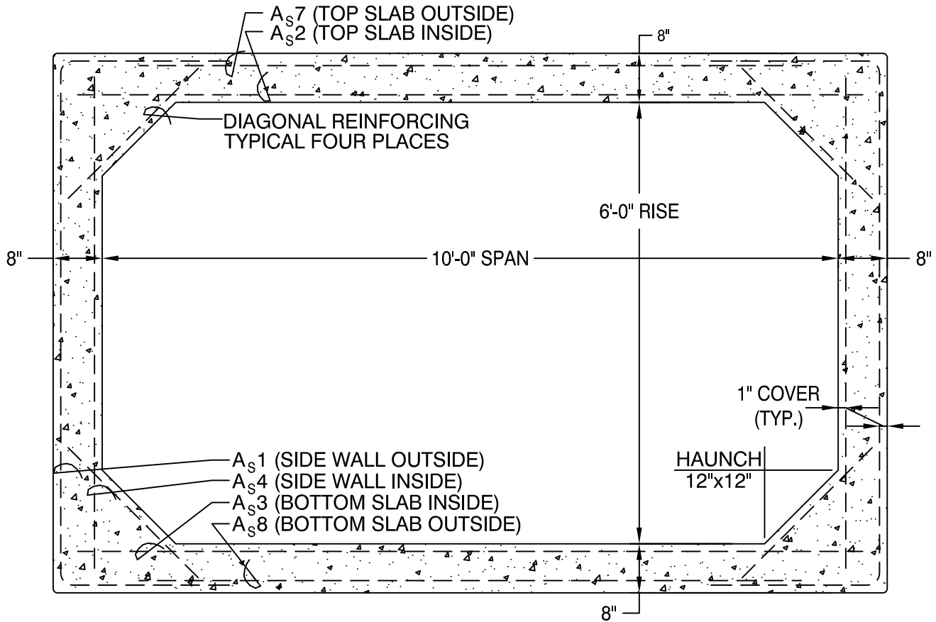
SECTION VIEW
