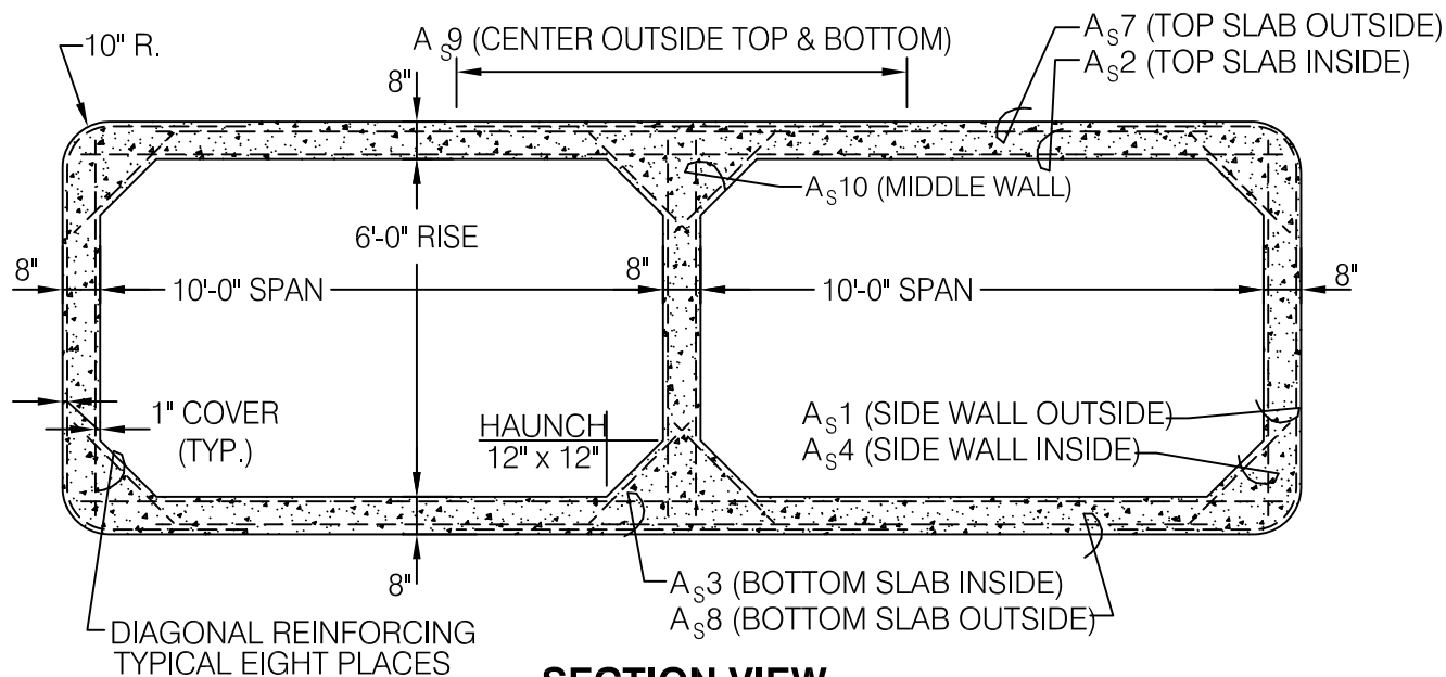
SECTION VIEW
