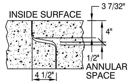
TYPICAL JOINT DETAIL
