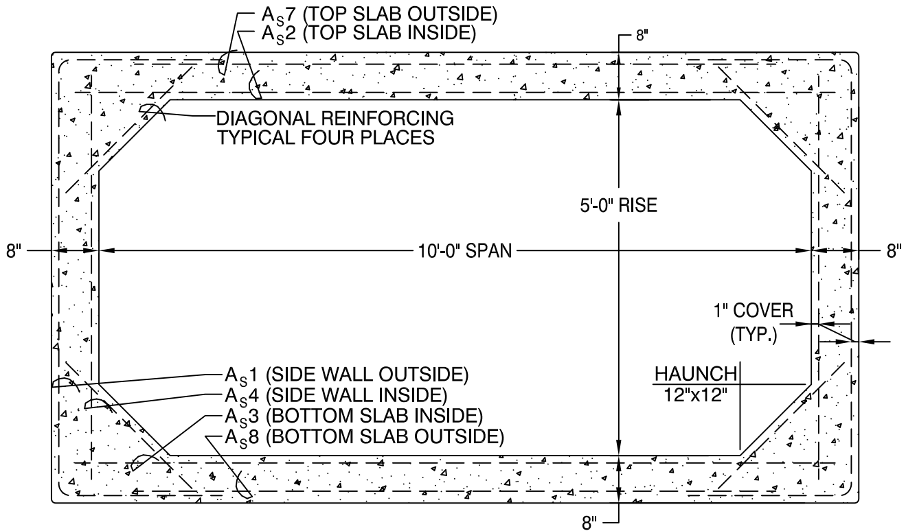
SECTION VIEW
