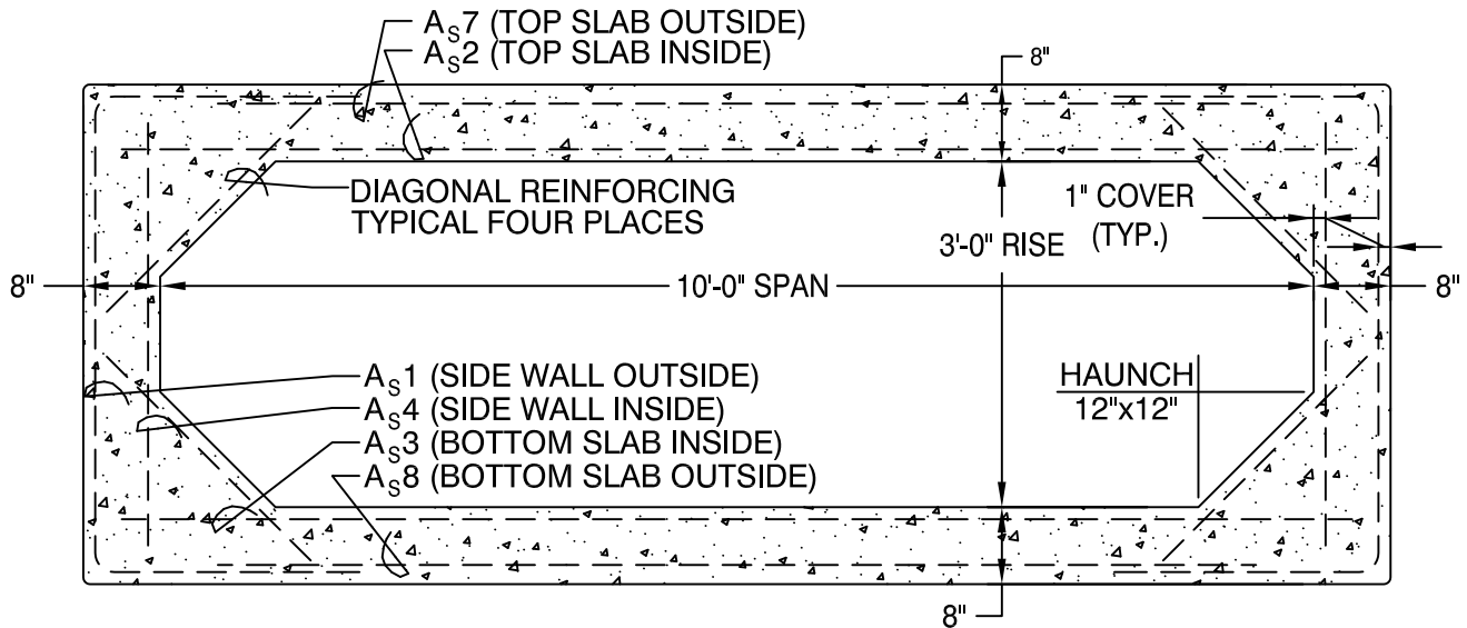
SECTION VIEW
